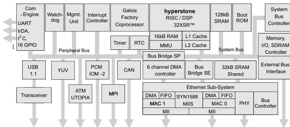
hyNet 32XS Block Diagram
